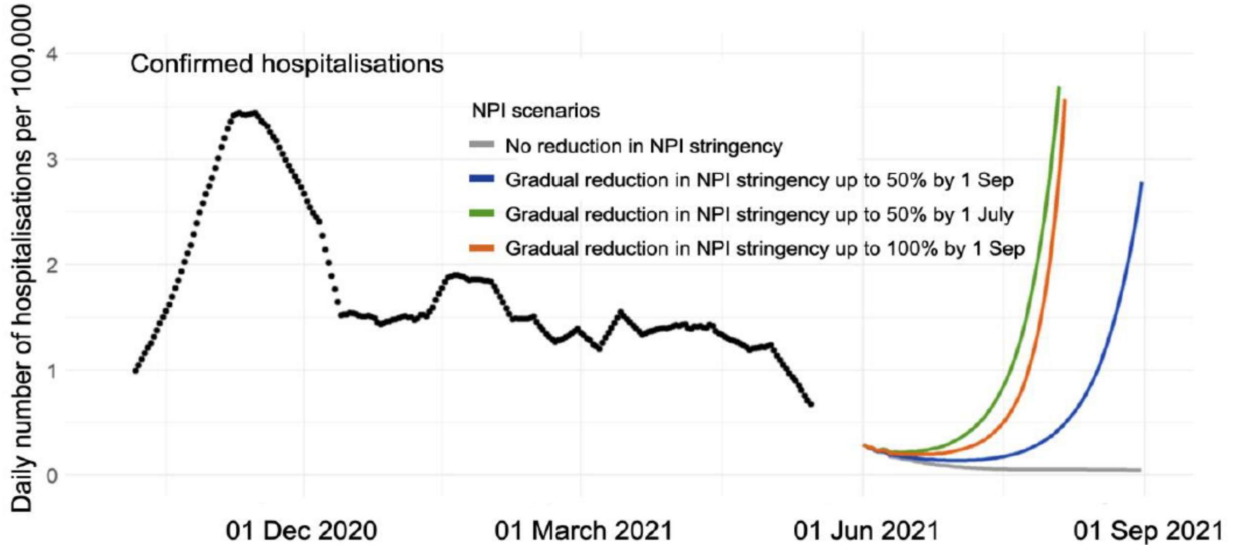
Figure 5. Estimation of possible changes in daily COVID-19 hospitalisation in the EU/EEA according to four NPI relaxation scenarios
